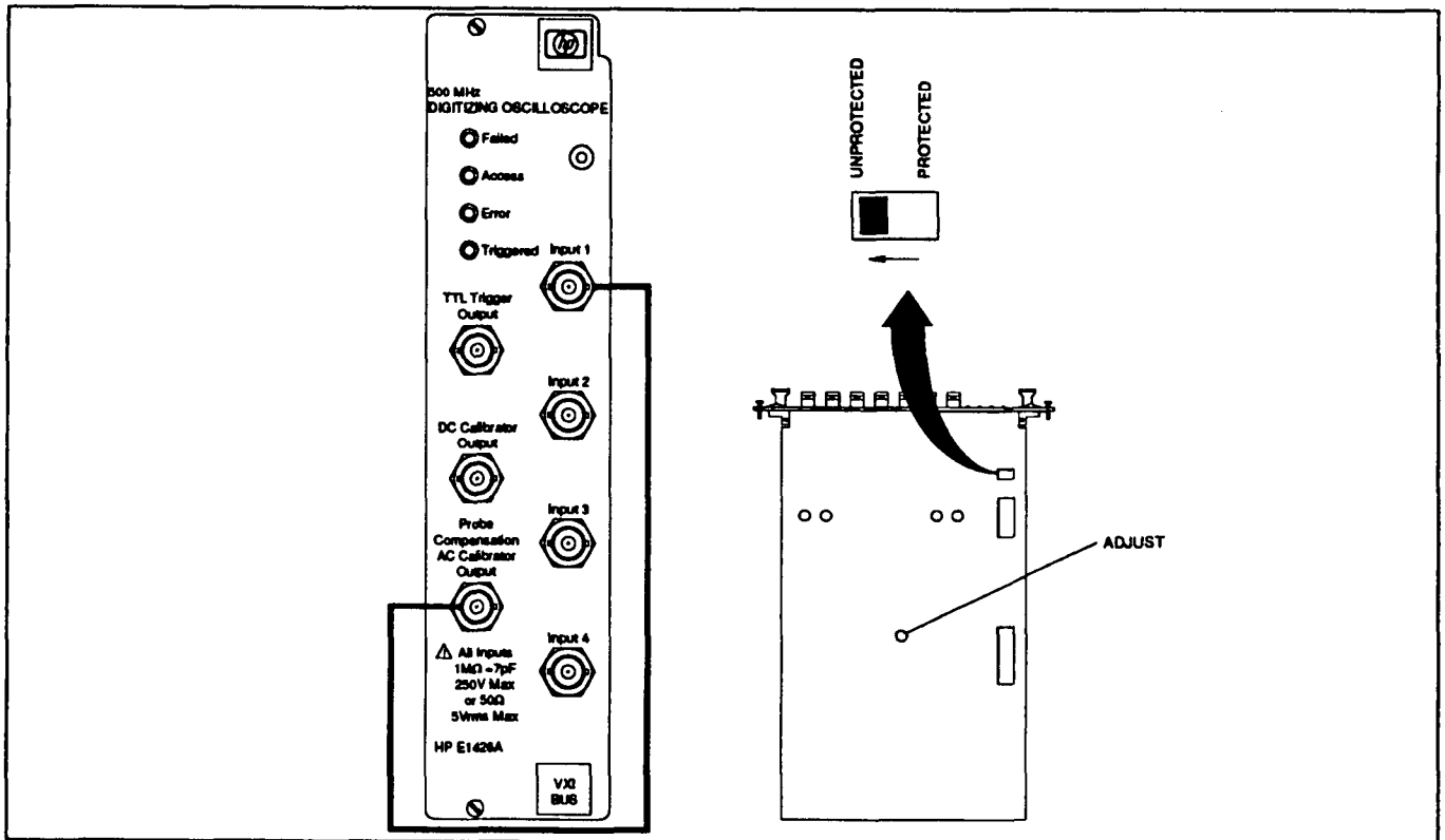
Figure 3-4. Example: Logic Trigger Calibration Setup
