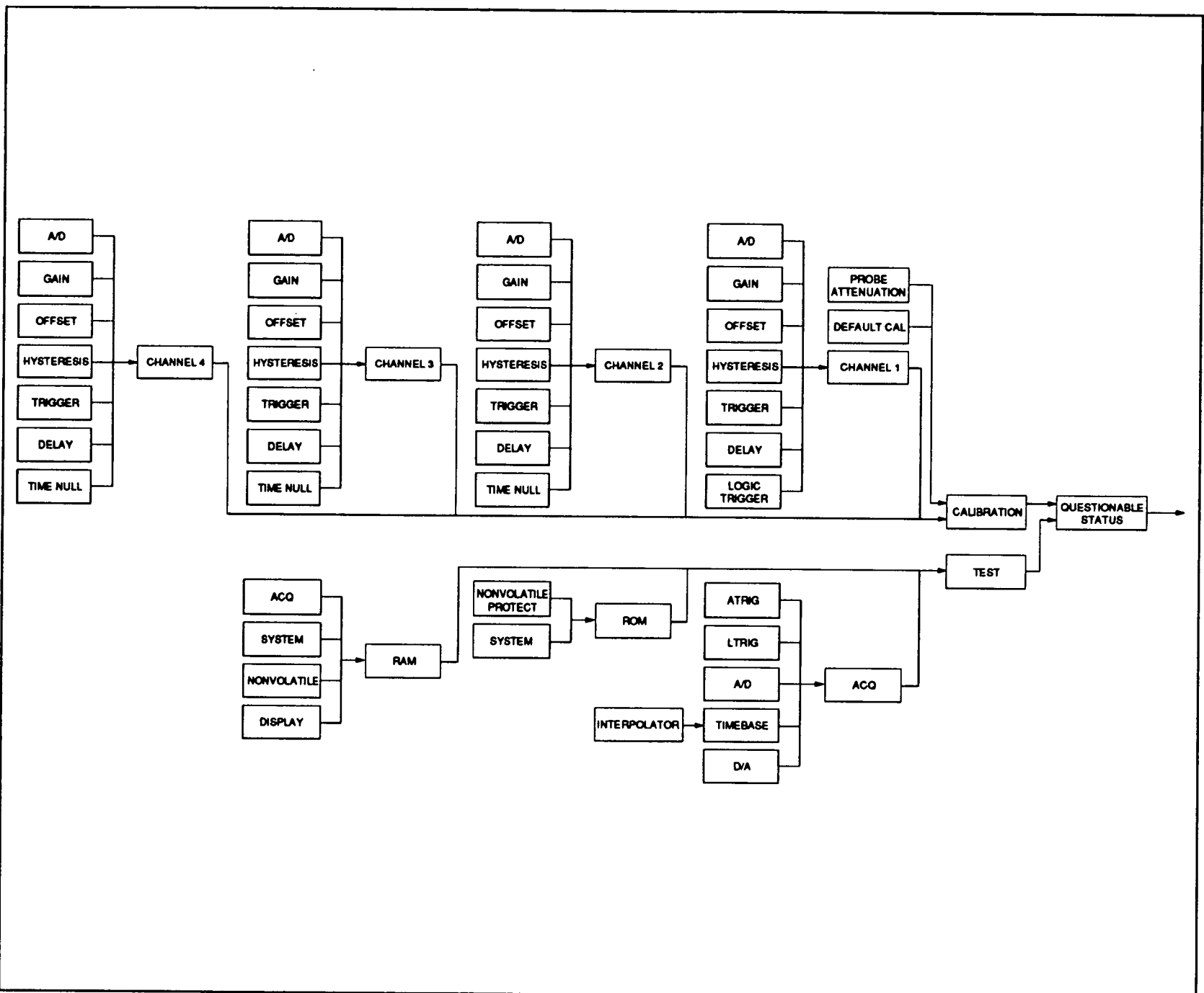
Figure 4-2. Oscilloscope Summary Questionable Data/Signal Register Subsystem
