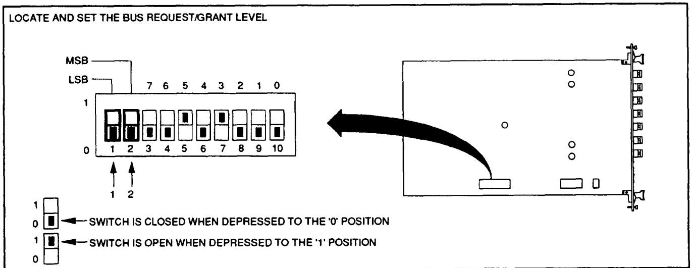
Figure 2-2. Bus Request/Grant Level Selection
